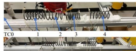
Initial experimental setup: closeup with TC locations numbered (top) and full view (bottom).
